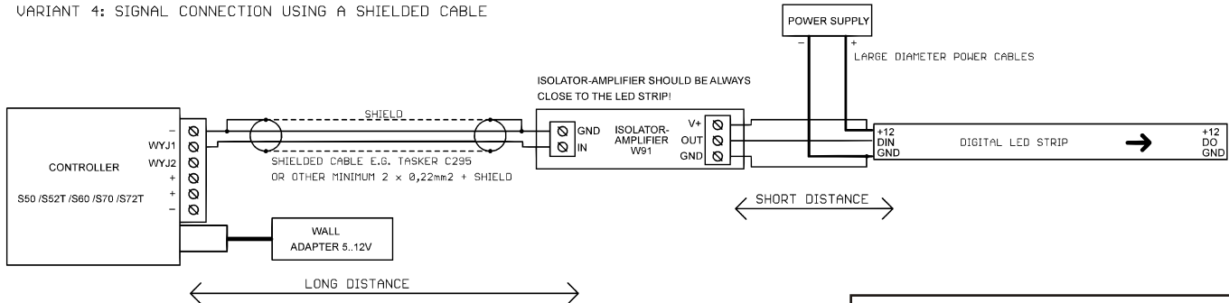
VARIANT 4: SIGNAL CONNECTION USING A SHIELDED CABLE
