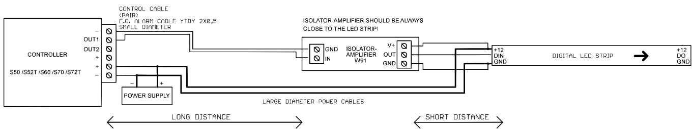
VARIANT 3: SEPARATE POWER SUPPLY FOR THE CONTROLLER (WALL ADAPTER)
